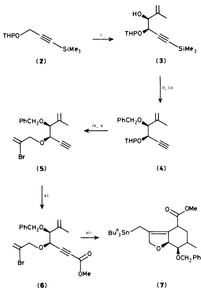
Scheme 2. Reagents and conditions: i, Bu t Li, Ti(OPr) i 4 , CH 2 =C(Me)CHO, -96 °C, tetrahydrofuran (THF), 80%; ii, NaOH–MeOH, 97%; iii, NaH, PhCH 2 Br, dimethoxyethane, 86%; iv, HCl–MeOH, 93%; v, CH 2 =C(Br)CH 2 Br, 50% NaOH(aq.), CH 2 Cl 2 , cetyltrimethylammonium bromide (20 mol %), 79%; vi, Bu n Li, MeOCOCl, -78 °C, 67%; vii, Bu n 3 SnH (2 equiv.), azoisobutyronitrile (AIBN) (10 mol %), C 6 H 6 , 80 °C, 43%. THP = tetrahydropyran-2-yl.
